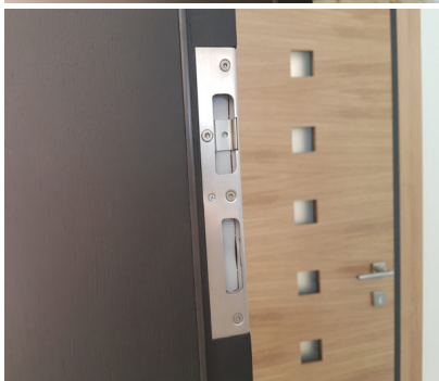
Caption 1b: ... or a simple striking plate against one with adjustment function. Photo: BaSys
